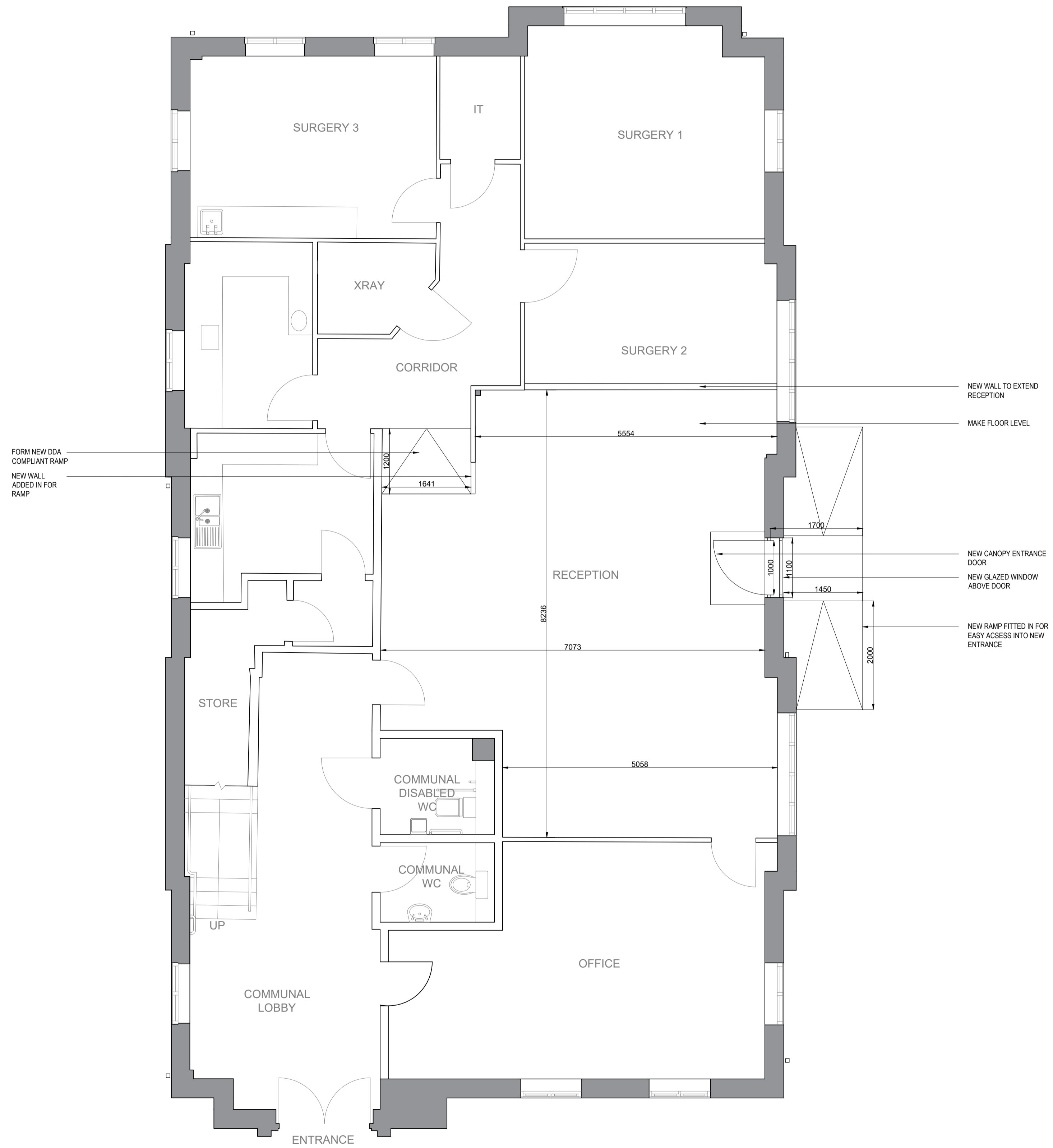
01 PROPOSED GROUND FLOOR CONSTRUCTION Scale 1:50
